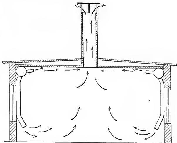
FIG. 7. TYPICAL DUCT ARRANGEMENT FOR DYE HOUSES
